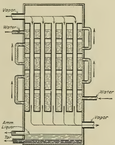
Fig. 60.—Water Condenser.
